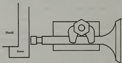
FIGURE 10-17. Grinding a valve tip.
